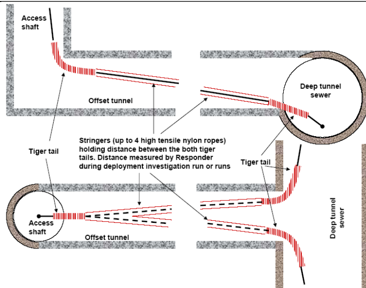
Figure 3 – Plan & Elevation View Showing Deployment of “Tiger Tails”
