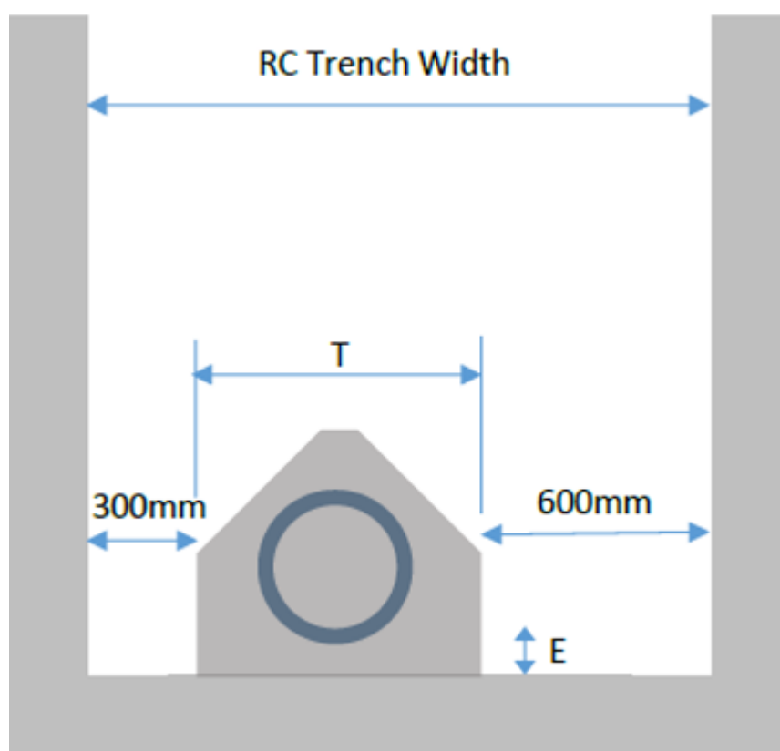
Figure 2: RC trench Width for Sewer Depth > 3 m or Diameter > 300 mm (Fully Haunch Type D)
