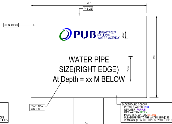
STANDARD DESIGN TO MARK OUT THE RIGHT EDGE OF WATER PIPES \geq 1200 MM DIA.
