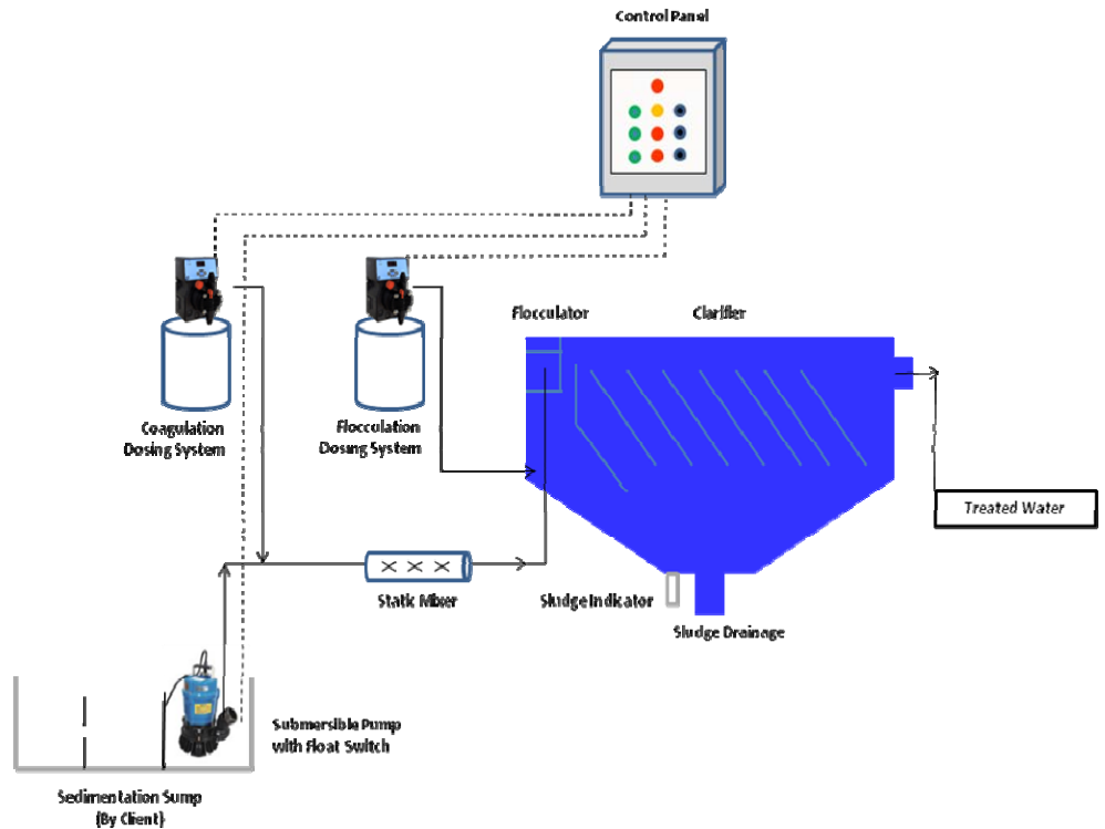
Model: FP-WW-40, Capacity: 40m 3 /hr
