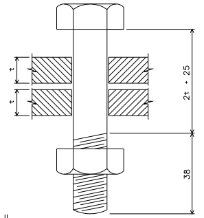
16 DIA. BOLT NO WASHER TO BE USED SCALE 1:1
