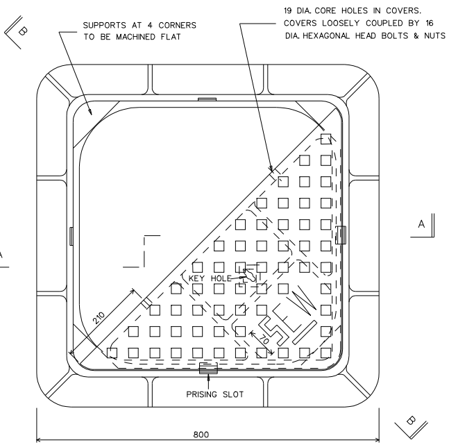
PLAN HALF COVER REMOVED SCALE 1:5
