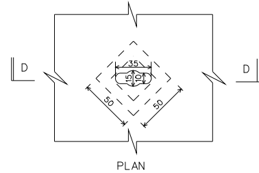
PLAN DETAIL OF KEYHOLE SCALE 1:2
