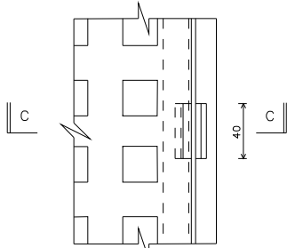
PLAN DETAIL OF PRISING SLOT SCALE 1:2
