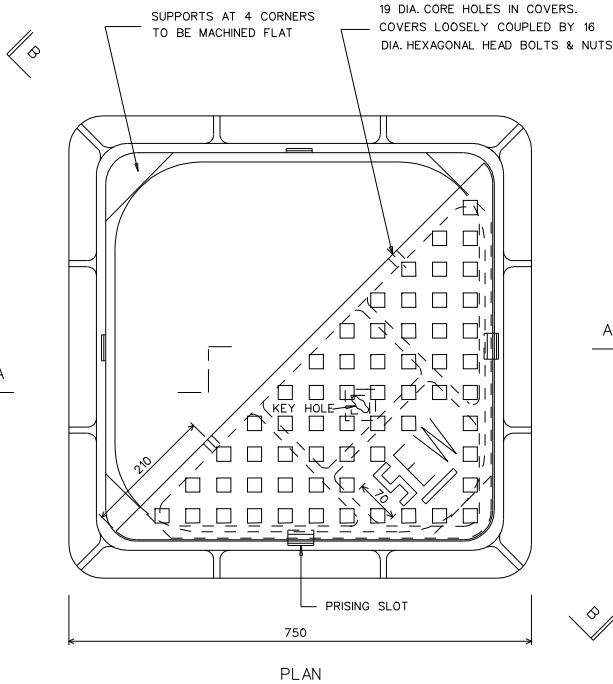
PLAN HALF COVER REMOVED SCALE 1:5
