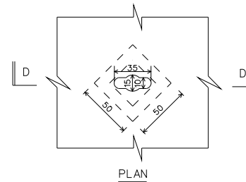
DETAIL OF KEYHOLE SCALE 1:2
