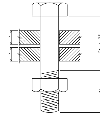
M16 BOLT NO WASHER TO BE USED
