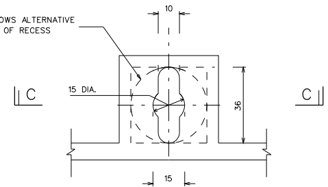
DETAILS OF KEYHOLE
