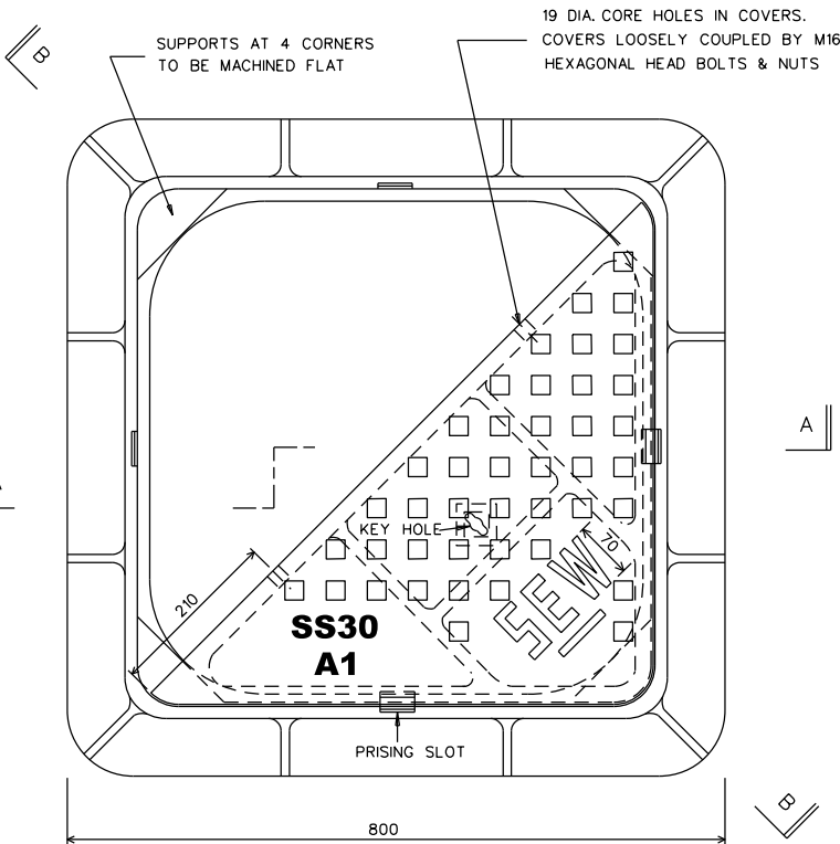
PLAN HALF COVER REMOVED SCALE 1:5
