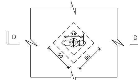
DETAIL OF KEYHOLE SCALE 1:2
