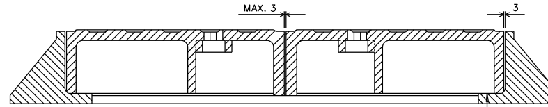
SECTION B - B
