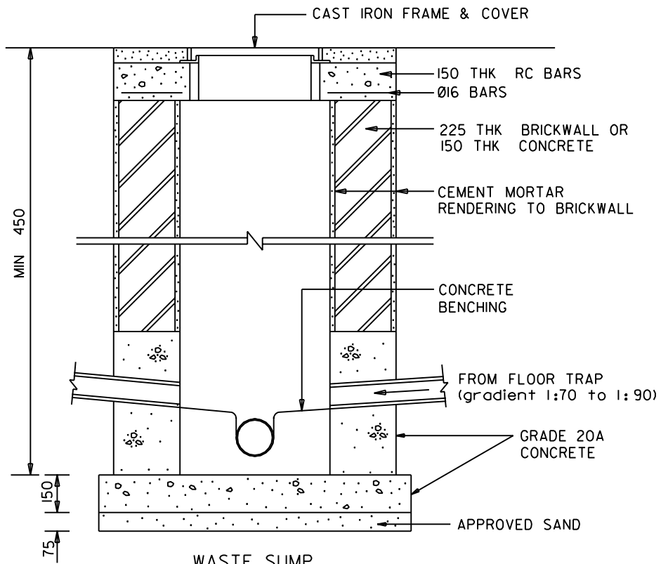
WASTE SUMP SCALE 1 : 20
