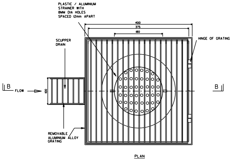
DETAILS OF FLOOR WASTE (FW)
