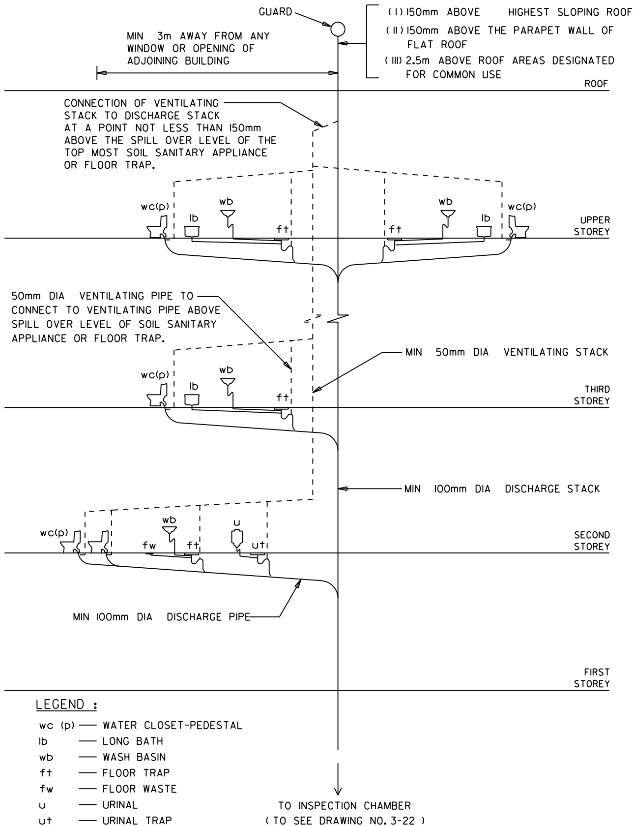
FULLY VENTILATED SYSTEM WITH VENTILATING ARRANGEMENT FOR SIX-STOREY OR LOWER MULTI-STOREY BUILDINGS
