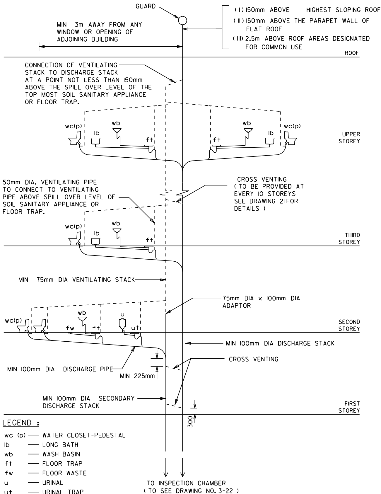
FULLY VENTILATED SYSTEM WITH VENTILATING ARRANGEMENT FOR SEVEN-STOREY OR HIGHER MULTI-STOREY BUILDINGS
