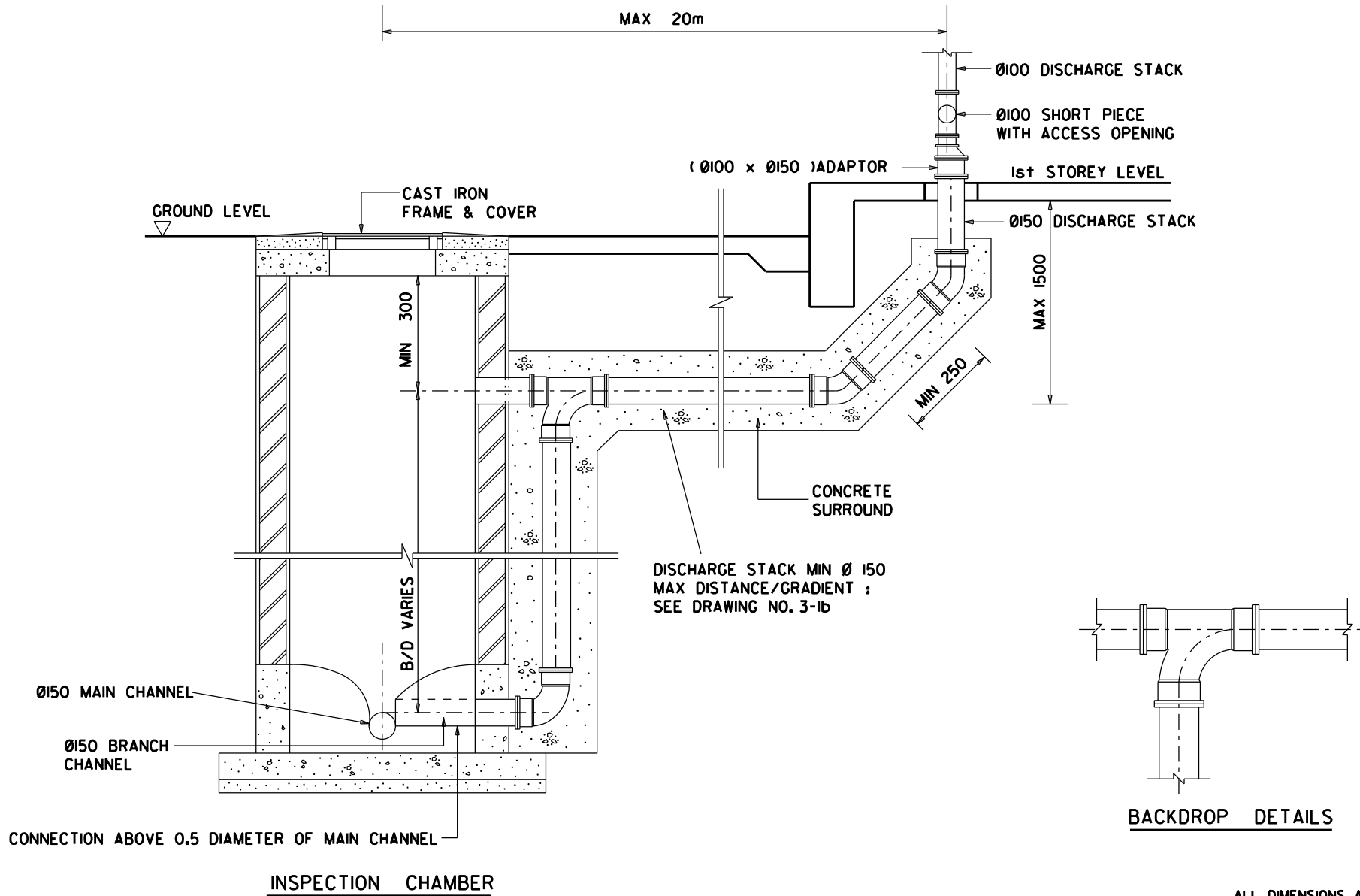
DISCHARGE STACK CONNECTION WITH BACKDROP TO INSPECTION CHAMBER
