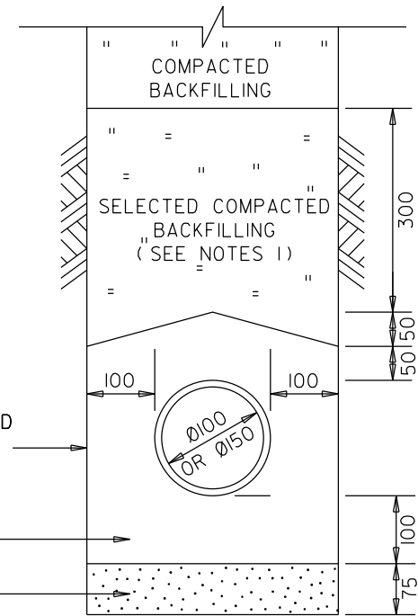
ON FIRM GROUND (TYPE '3' BEDDING)
