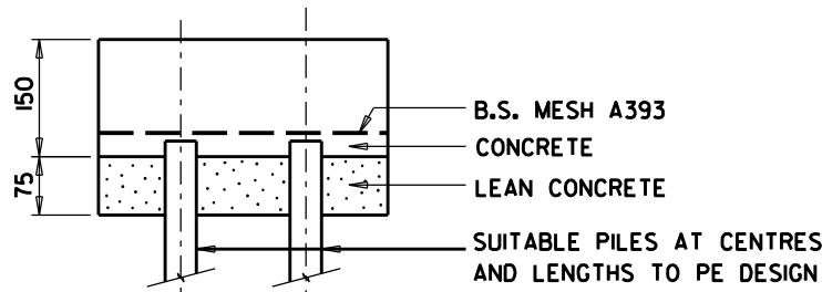
ON SOFT OR YIELDING GROUND ( PILES ARE REQUIRED )
