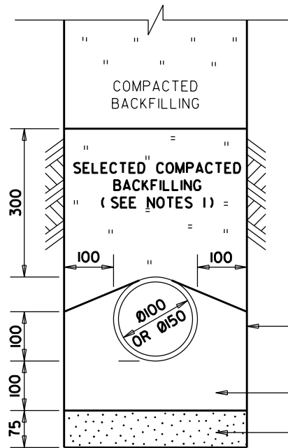
ON FIRM GROUND ( TYPE '2' BEDDING )
