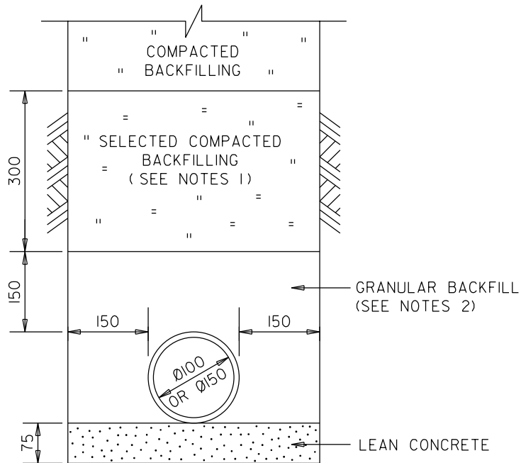
ON FIRM GROUND (TYPE '1' BEDDING)
