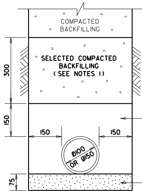
ON FIRM GROUND ( TYPE '1' BEDDING )
