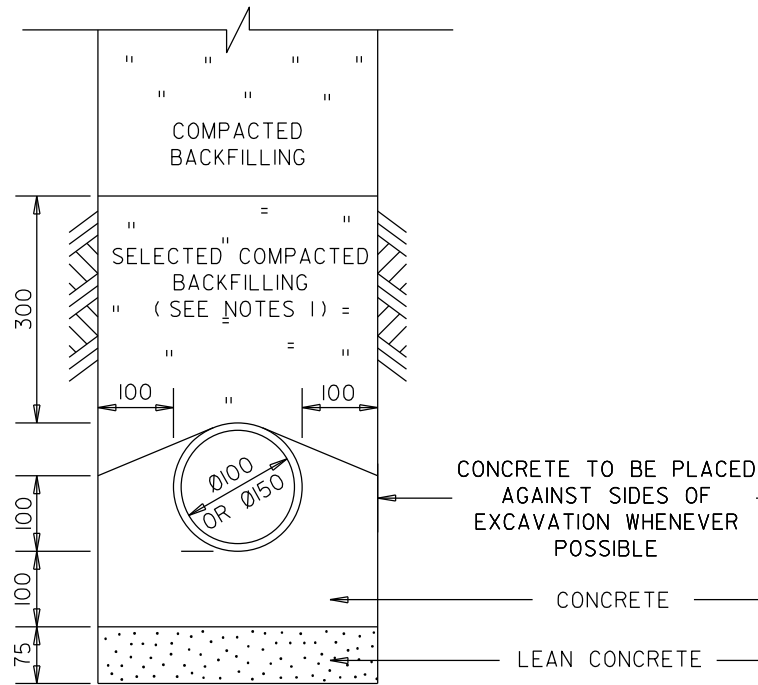
ON FIRM GROUND (TYPE '2' BEDDING)
