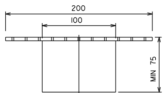
SCUPPER DRAIN (ELEVATION)
