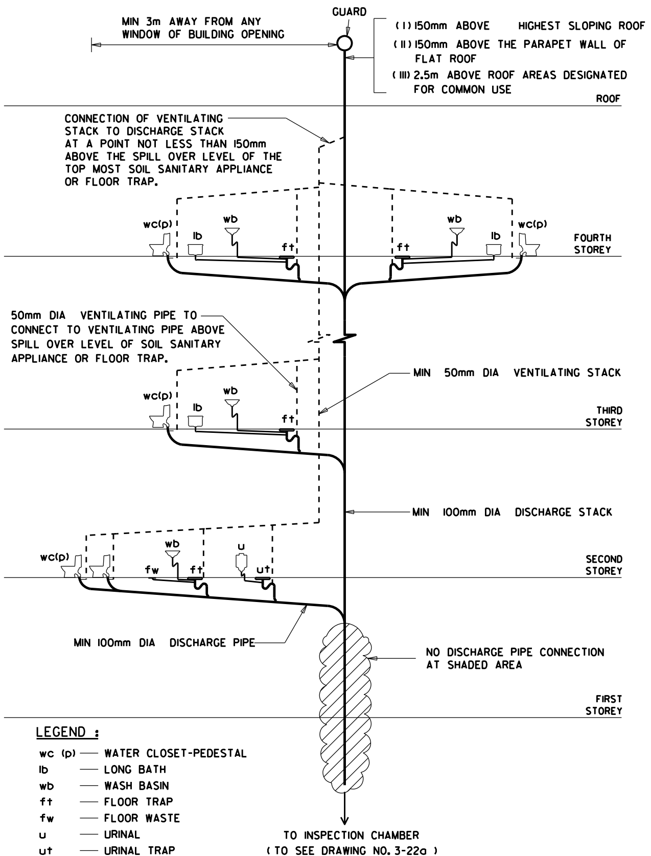
FULLY VENTILATED SYSTEM (WITH SINGLE STACK) FOR SINGLE LANDED HOUSING
