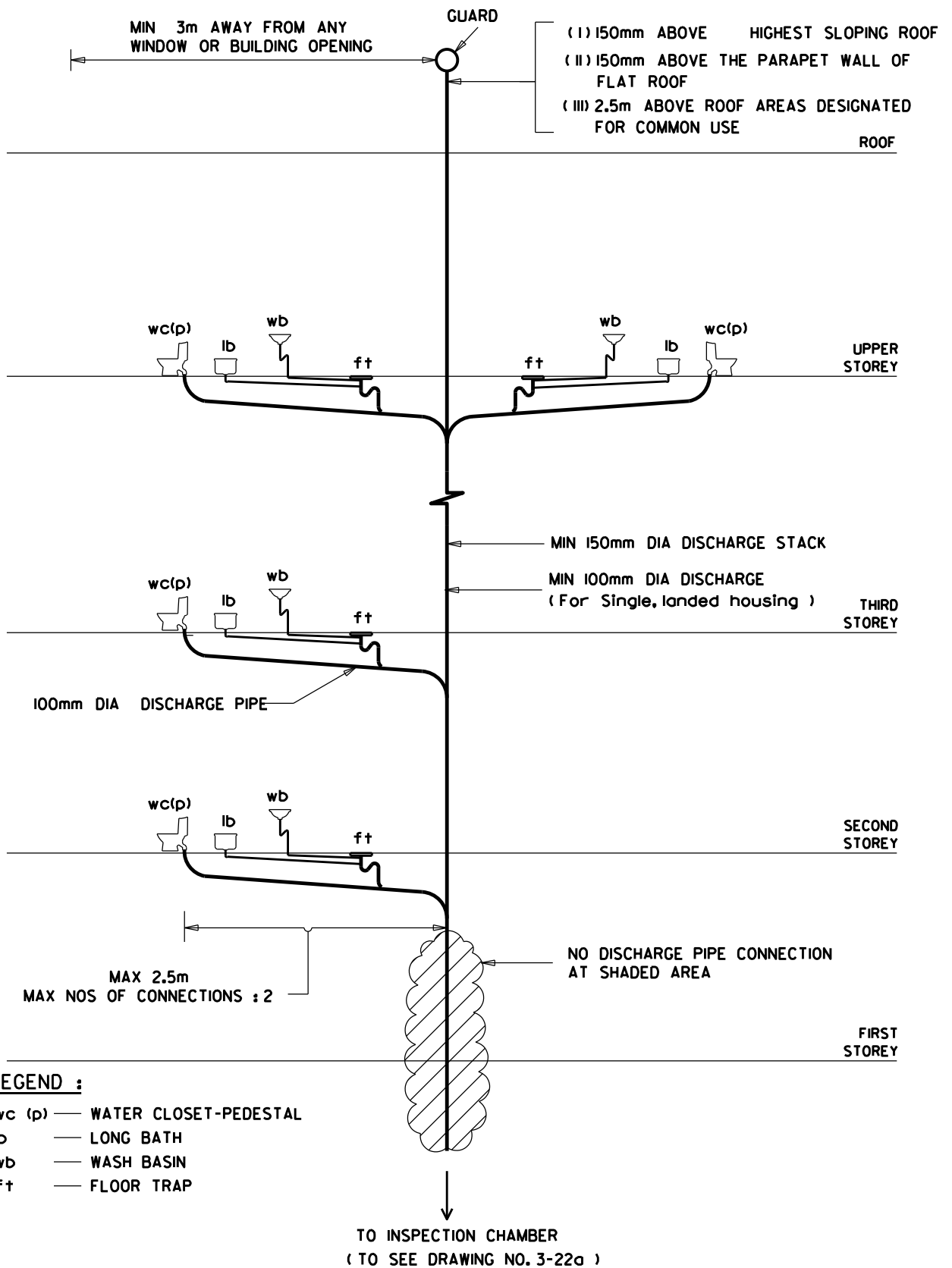
SINGLE STACK SYSTEM FOR BUILDINGS UP TO 6 STOREYS
