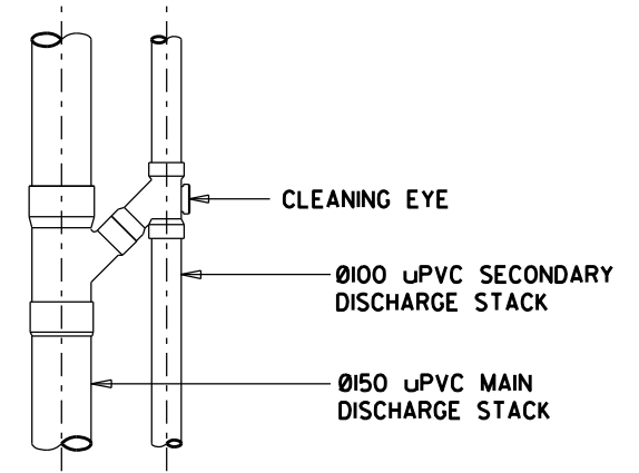
CROSS VENTILATING PIPE BETWEEN SECONDARY AND MAIN DISCHARGE STACKS
