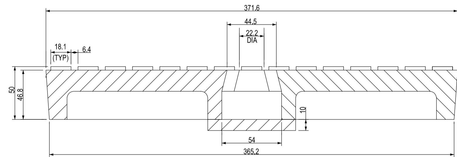
STANDARD SQUARE DUCTILE IRON (GRADE A1) MANHOLE FRAME AND COVER (FOR GROUND HYDRANT)
