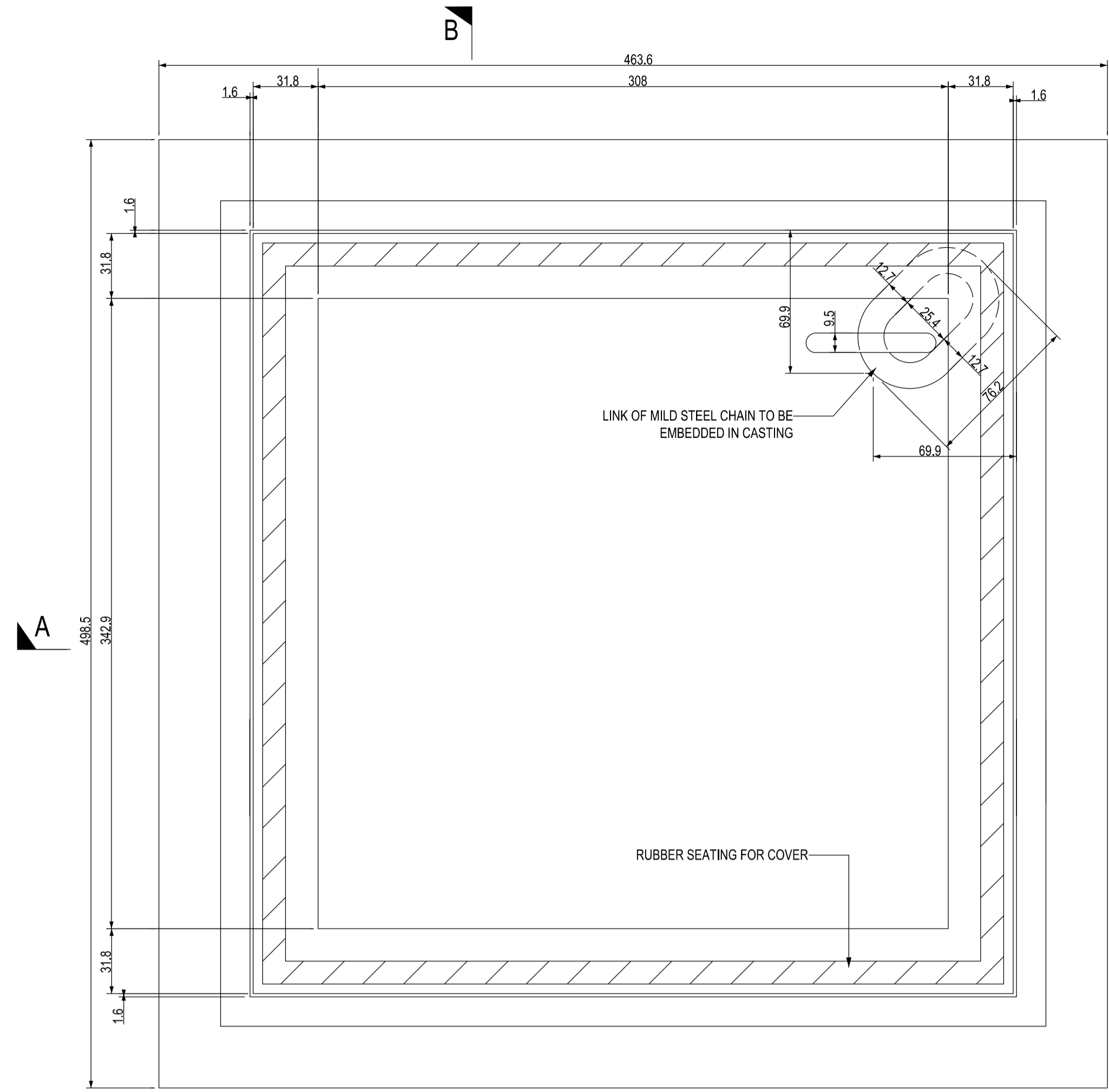
STANDARD SQUARE DUCTILE IRON (GRADE A1) MANHOLE FRAME AND COVER (FOR GROUND HYDRANT)
