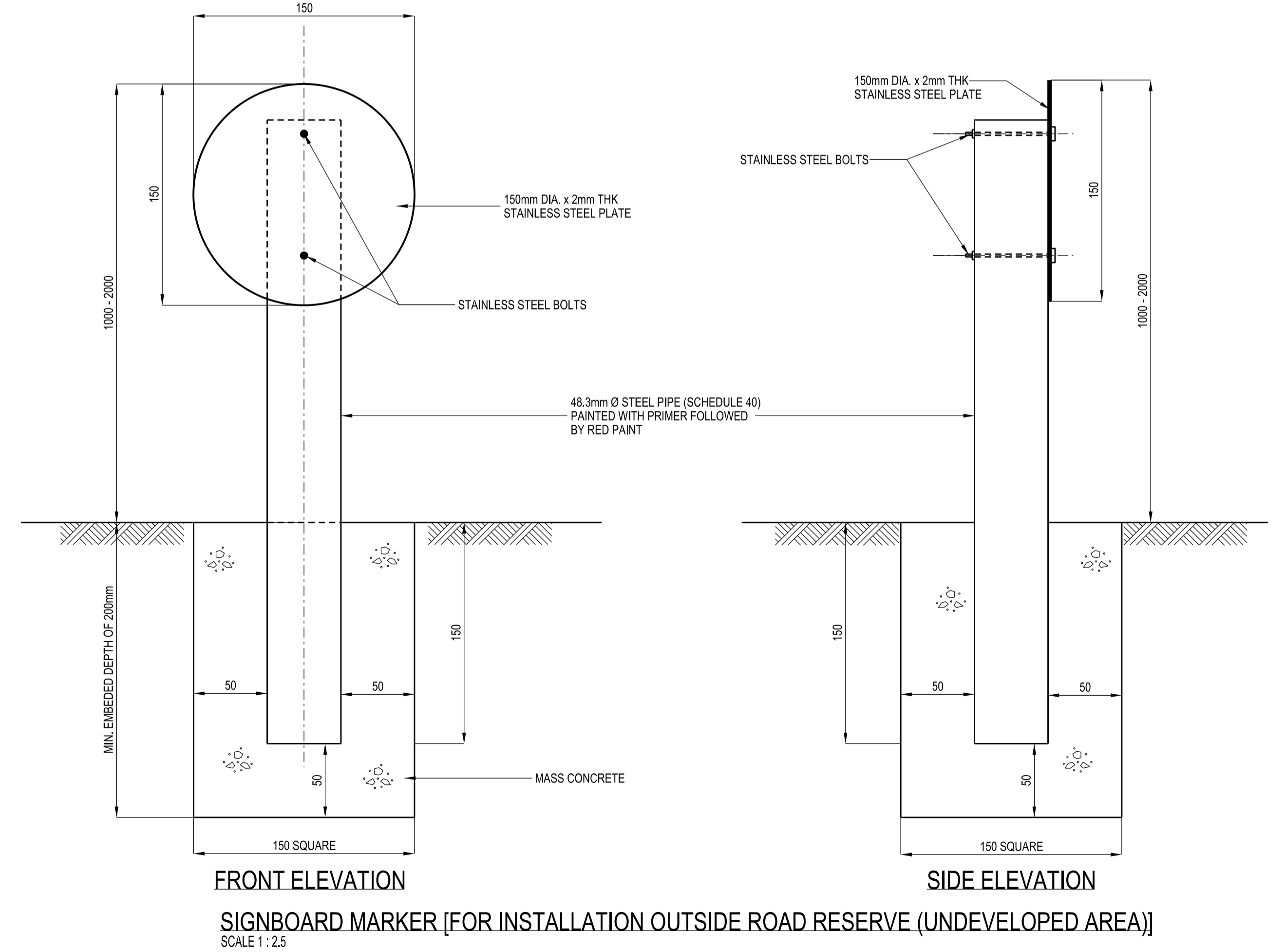
STAINLESS STEEL MARKER PLATE SCALE 1:2.5
