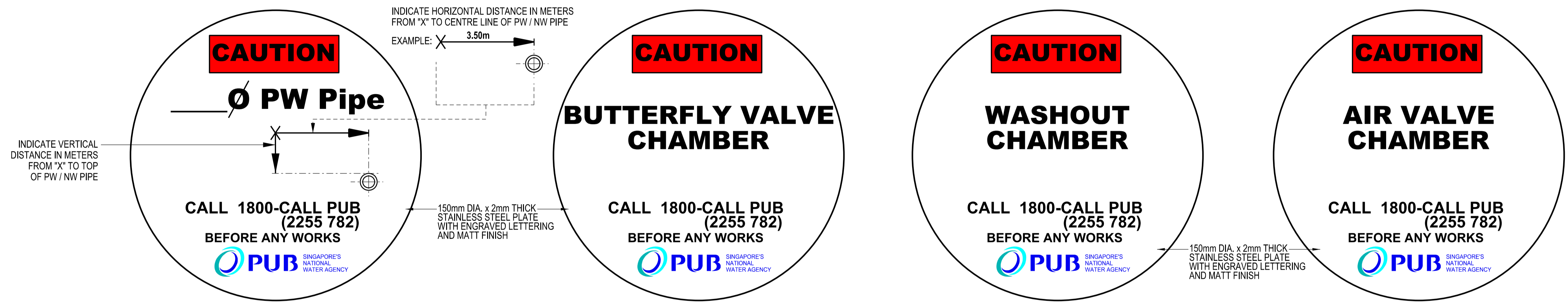
STAINLESS STEEL MARKER PLATE SCALE 1:2.5
