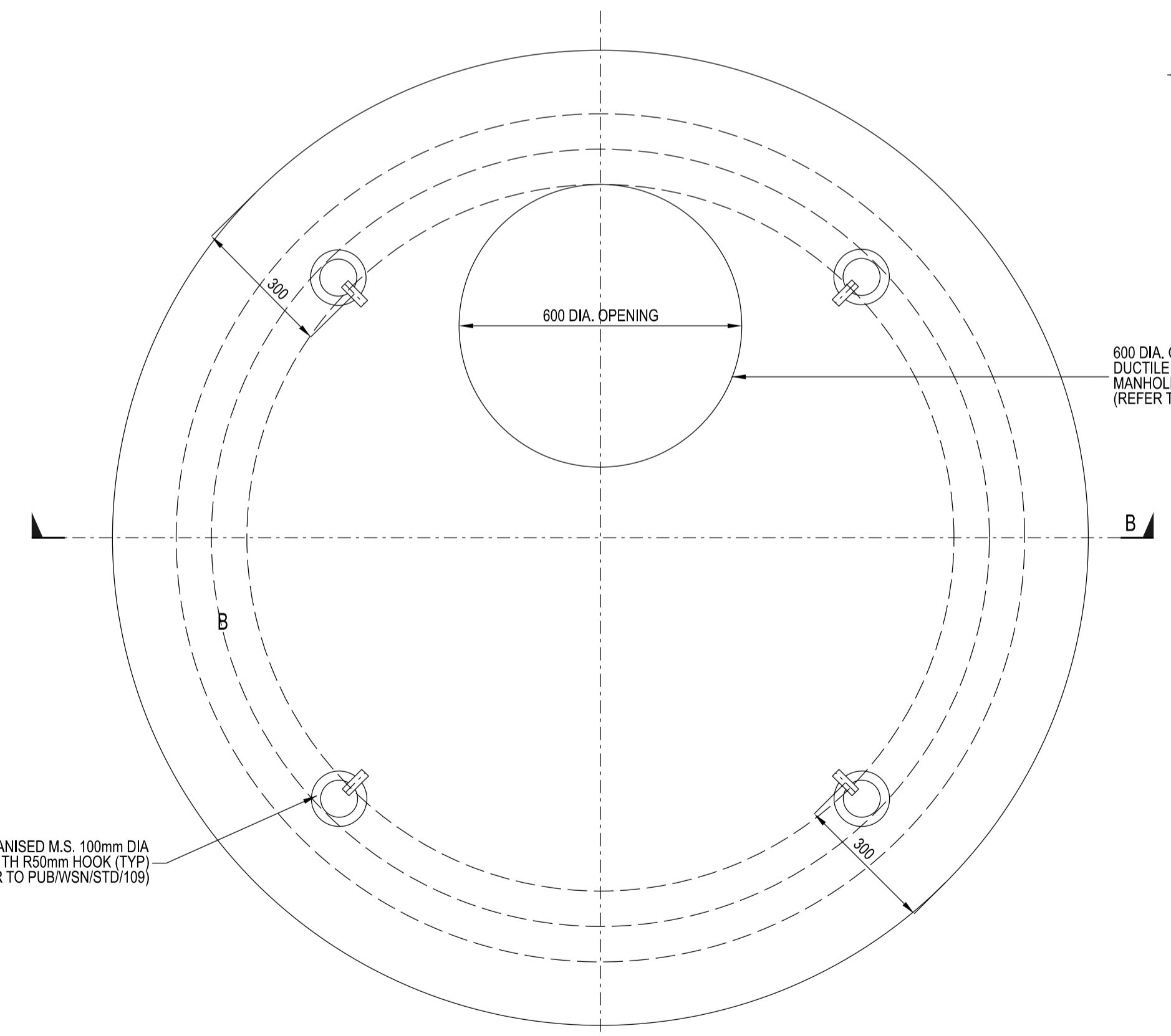
PLAN OF PRECAST R.C. COVER SLAB
