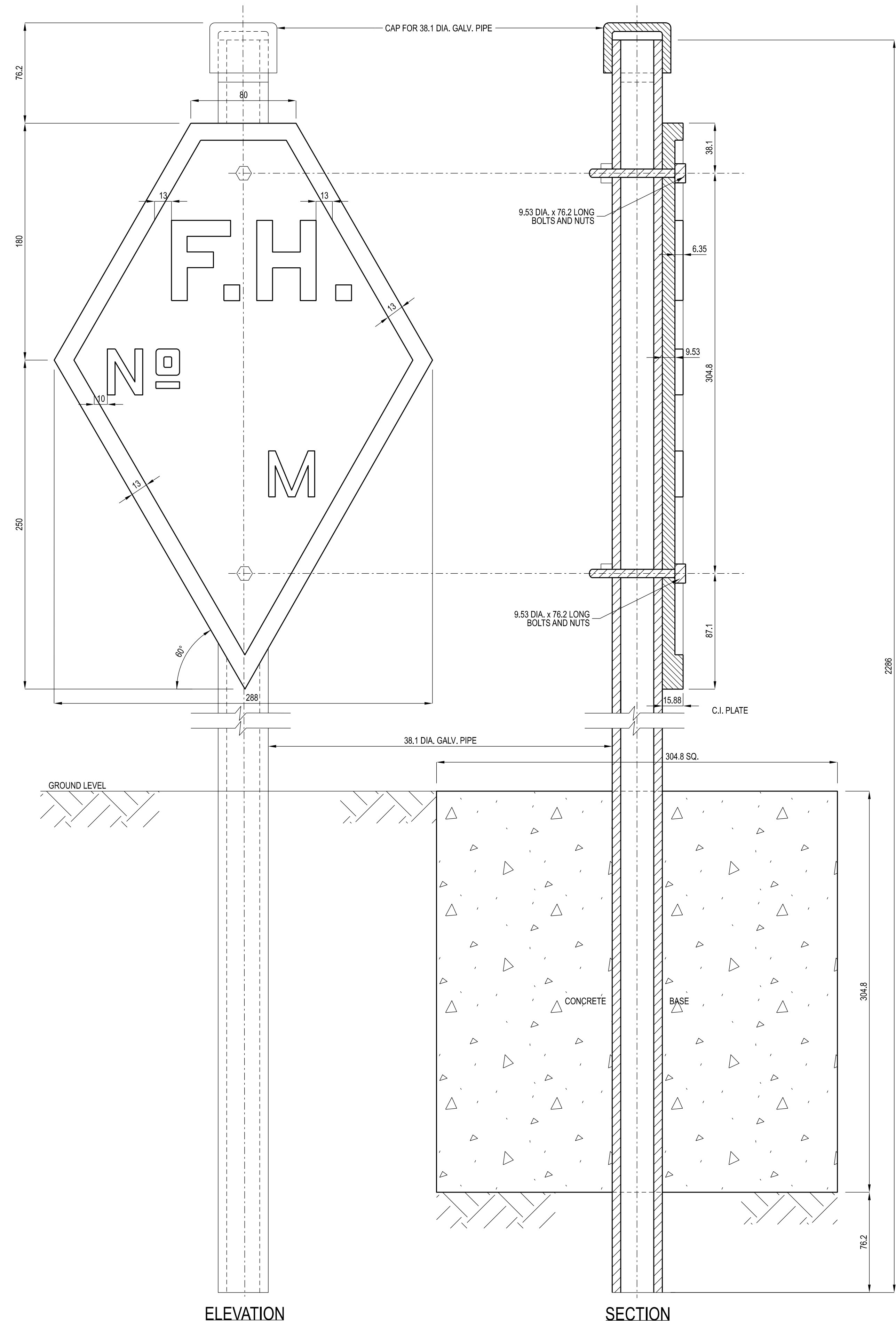
TYPICAL DETAIL OF INDICATOR PLATE SCALE 1:2
