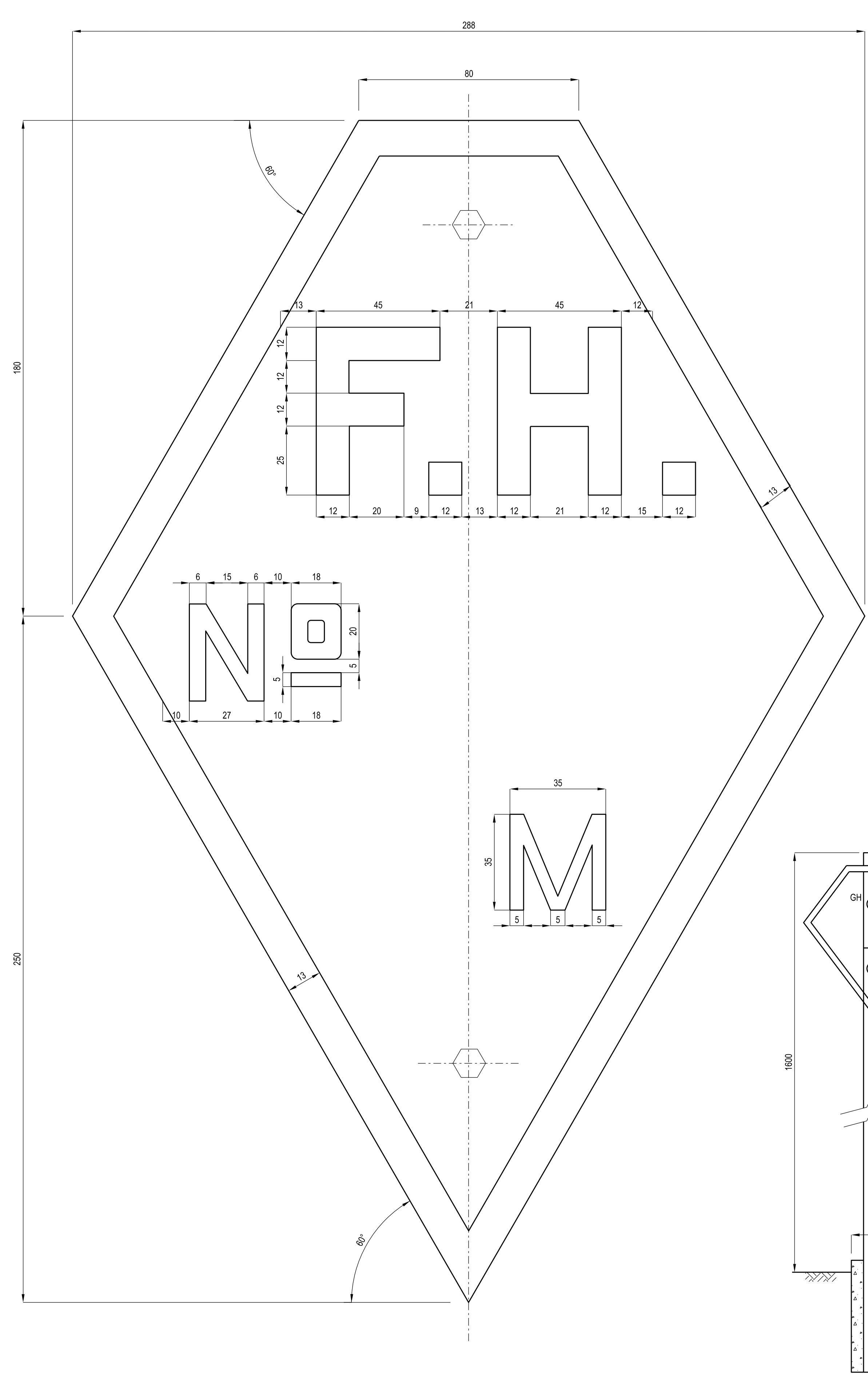
ENLARGED DETAIL OF INDICATOR PLATE SCALE 1:1
